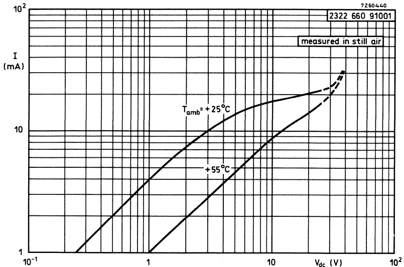
Fig. 2 Typical current/voltage characteristics.
