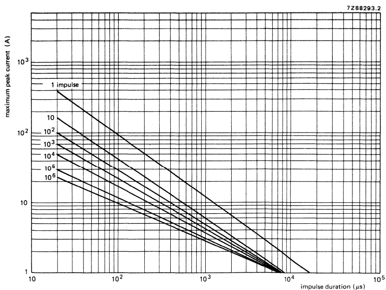
Fig. 14 Max. applicable transient current as a function of impulse duration, 50/460 V, 592 series.
