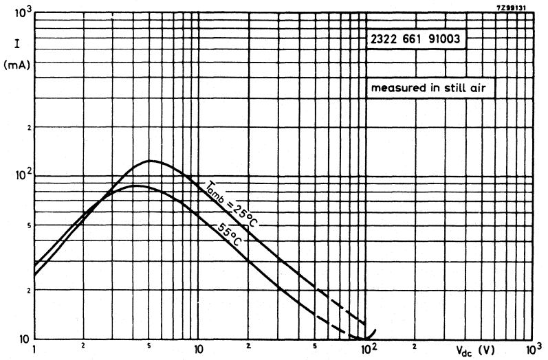
Fig. 5 Voltage/current characteristics.
