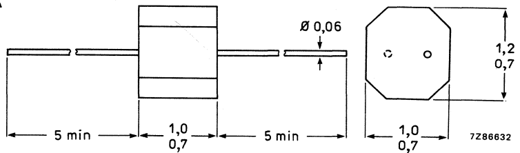
Fig. 1 version 2322 633 0....
