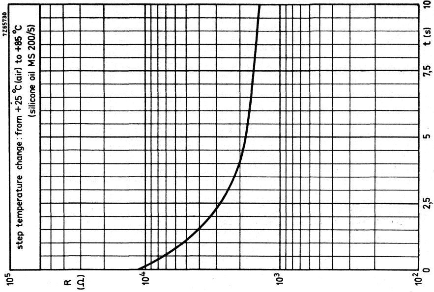
Fig. 5 Typical resistance/response time characteristics.
