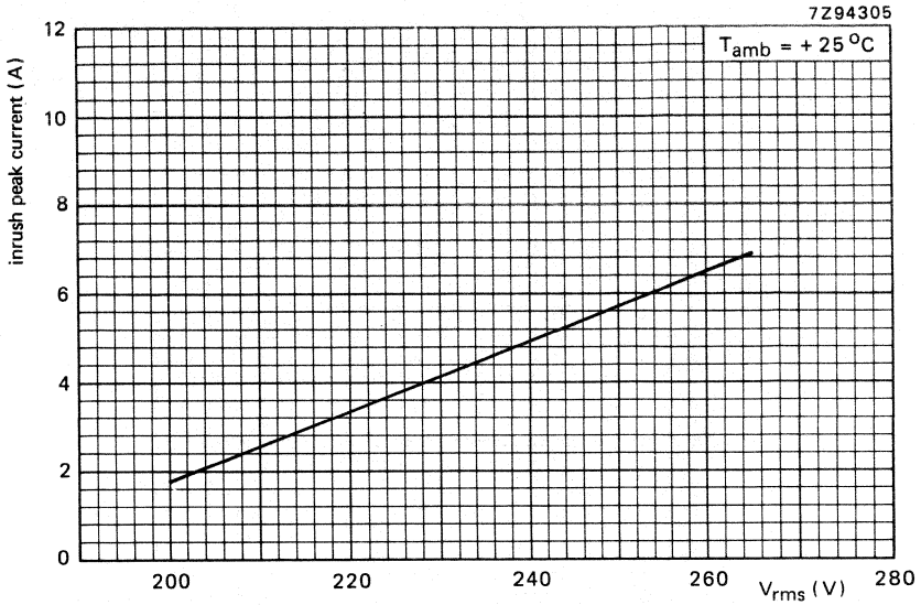
Fig. 6 Typical inrush peak current versus voltage characteristic.
