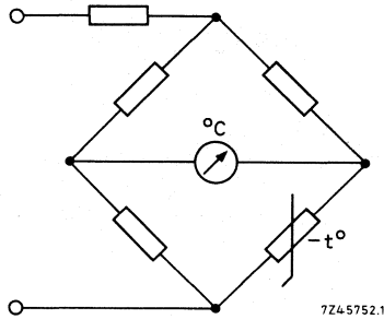
Fig. 12 Temperature measurement in industrial and medical thermometers.
