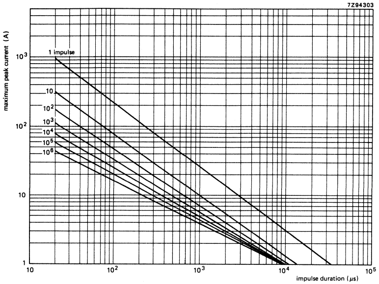
Fig. 19 Max. applicable transient current as a function of impulse duration, 30/40 V, 595 series.
