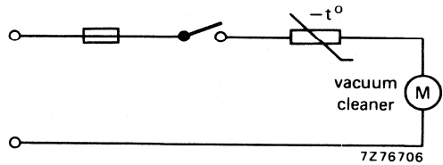
Fig. 17 Inrush current limiter, e.g. for protection of Si-diodes, fuses and switches.
