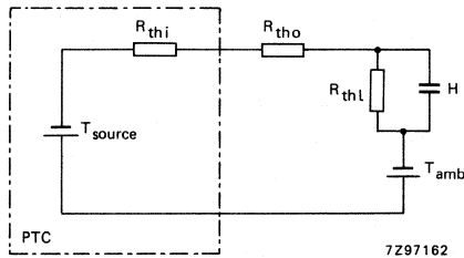
Fig. 2 Thermal equivalent circuit.
