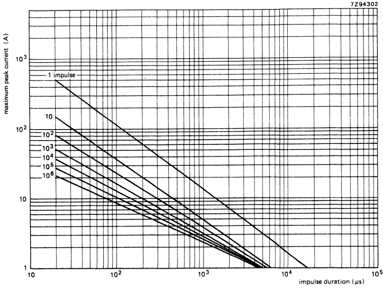
Fig. 17 Max. applicable transient current as a function of impulse duration, 30/40 V, 594 series.
