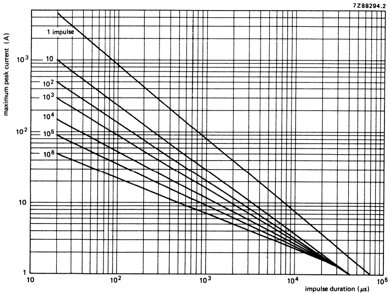
Fig. 20 Max. applicable transient current as a function of impulse duration, 50/460 V, 595 series.
