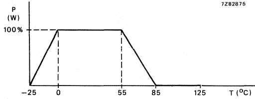
Fig. 4 Derating curve.
