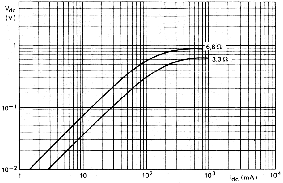
Fig. 5 Typical voltage/current characteristic, T_{amb} = +25\text{ }^{\circ}\text{C} , still air.
