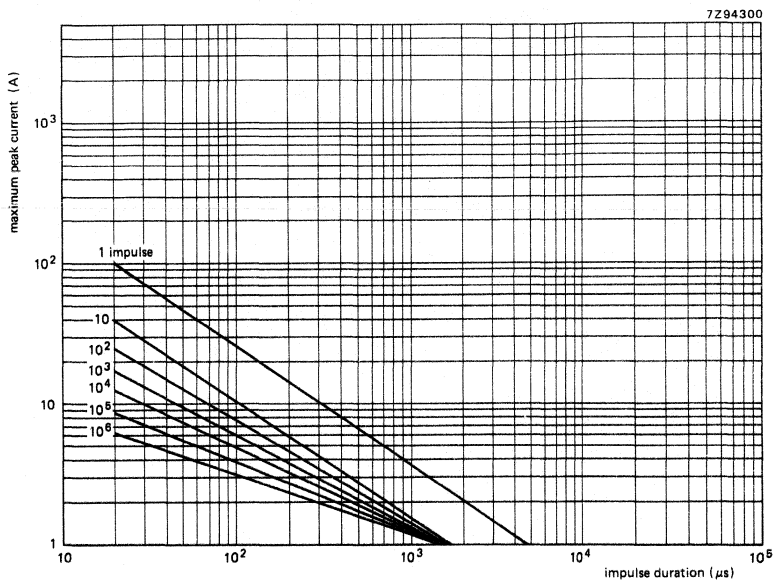
Fig. 13 Max. applicable transient current as a function of impulse duration, 30/40 V, 592 series.
