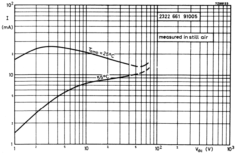
Fig. 7 Voltage/current characteristics.
