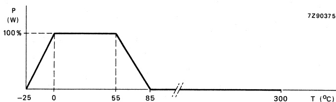
Fig. 2 Derating curve.
