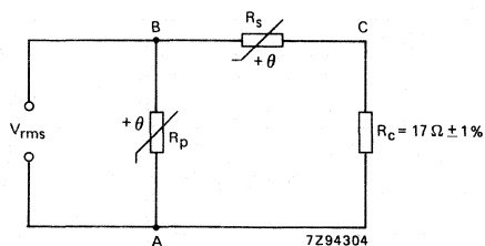
Fig. 2 Measuring circuit.
