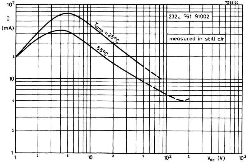
Fig. 4 Voltage/current characteristics.
