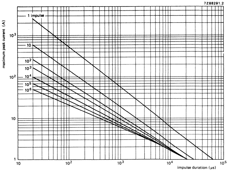
Fig. 18 Max. applicable transient current as a function of impulse duration, 50/460 V, 594 series.
