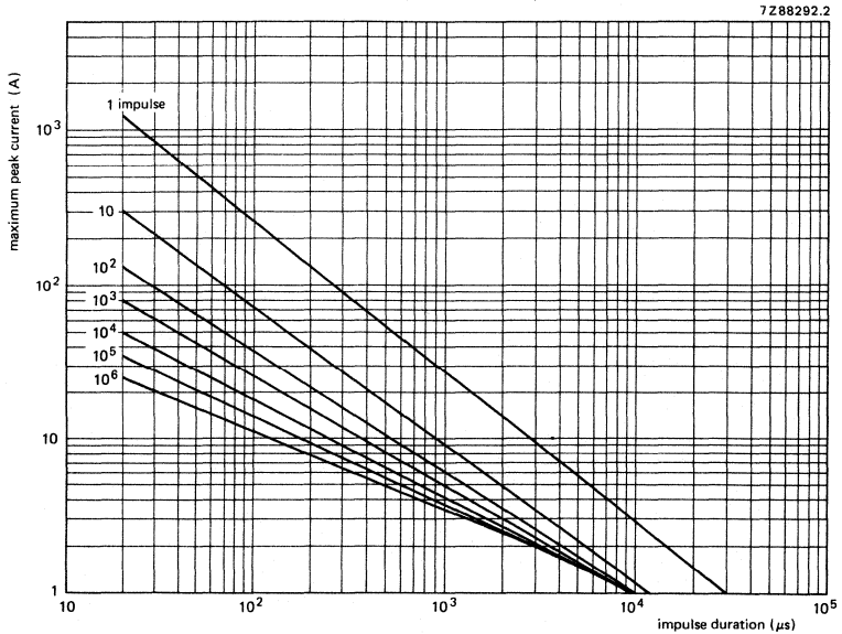
Fig. 16 Max. applicable transient current as a function of impulse duration, 50/460 V, 593 series.
