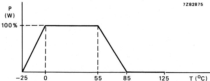
Fig. 2 Derating curve.
