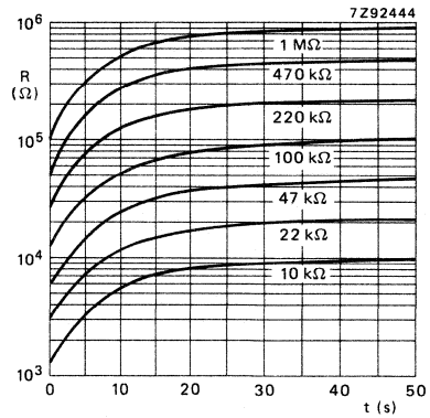
Fig. 6 Typical resistance/cooling time characteristics. Measured in still air at 25 °C. T_{start} = 85 °C.
