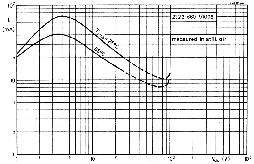
Fig. 8 Typical voltage/current characteristics.
