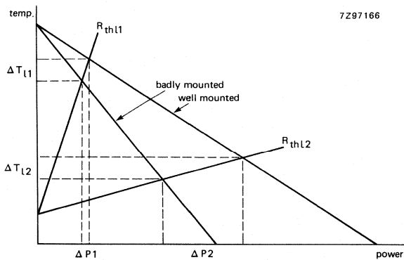
Fig. 6 Influence of mounting method.
