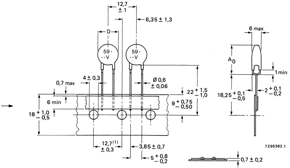
Fig. 6 Types 2322 593 3...2 on tape, D = 9 \text{ max} , A_0 = 13 .
