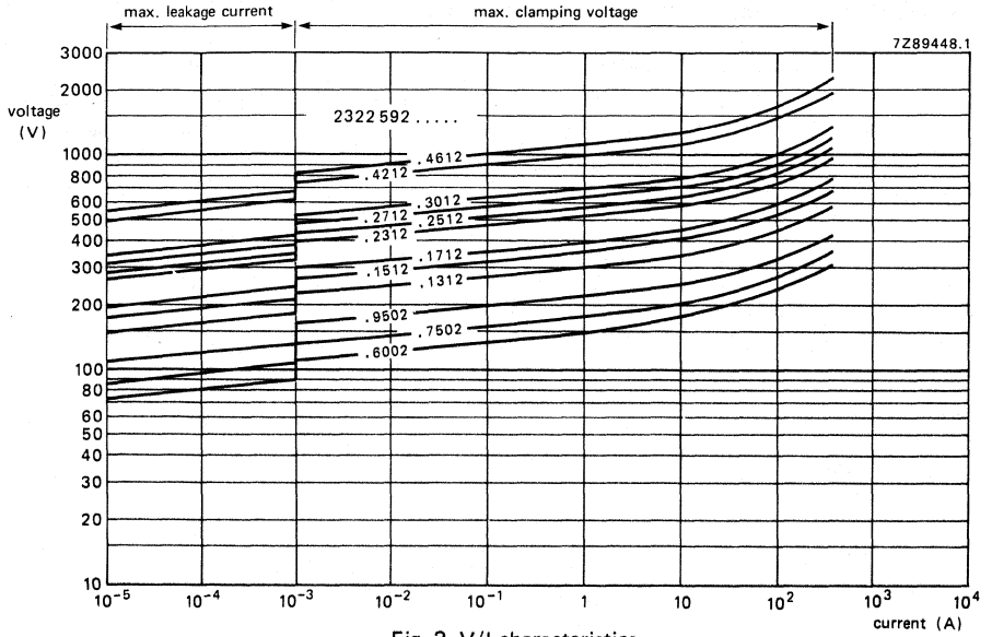
Fig. 2 V/I characteristics.
