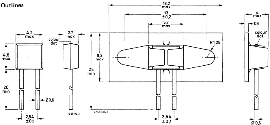
Fig.1 Type 2322 640 90013.
