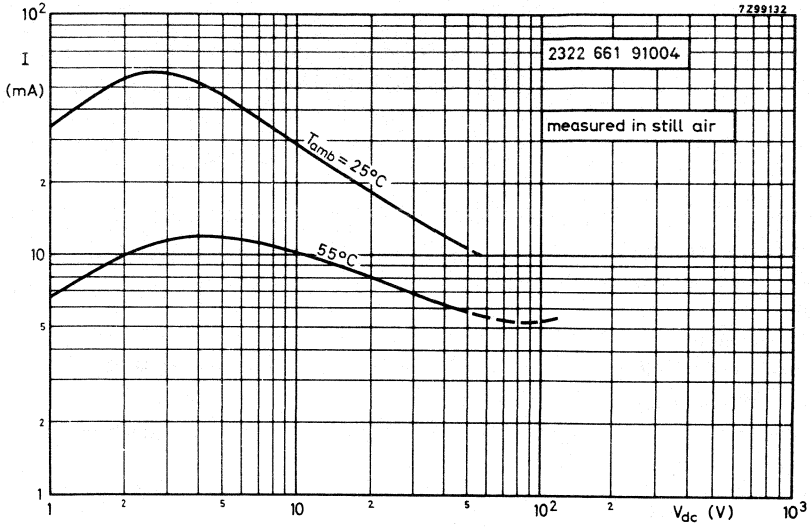
Fig. 6 Voltage/current characteristics.
