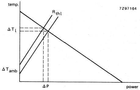
Fig. 4 Influence of ambient temperature.
