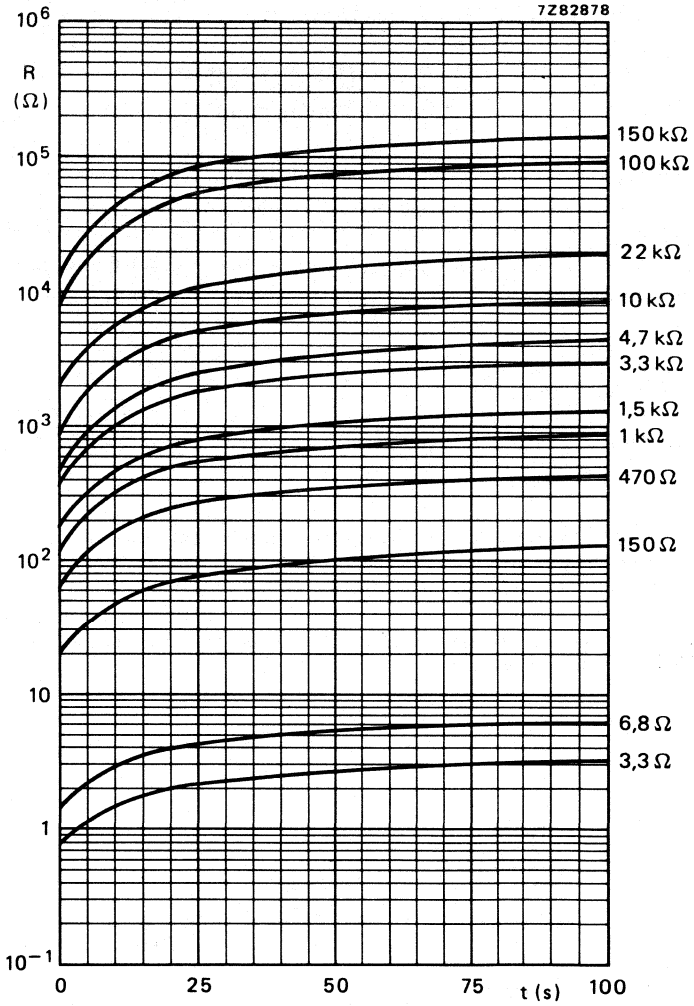
Fig. 8 Typical resistance/cooling time characteristic, T_{\text{amb}} = +25^\circ\text{C} , still air, T_{\text{start}} = +85^\circ\text{C} .
