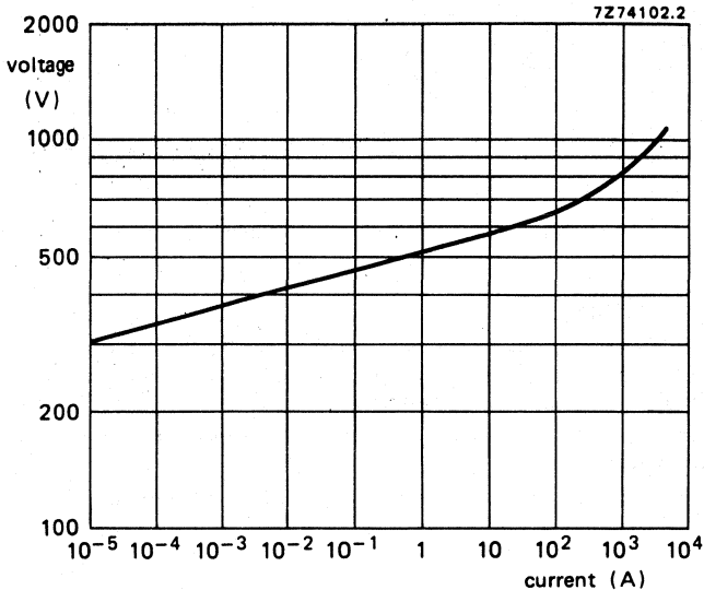
Fig. 9 Typical V/I characteristic of ZnO varistor 2322 595 62512 and 2322 595 62516 for 220 V mains supply.
