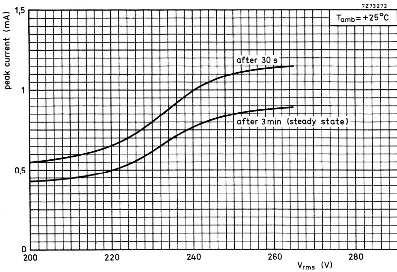
Fig. 7 Typical peak current versus voltage characteristics.
