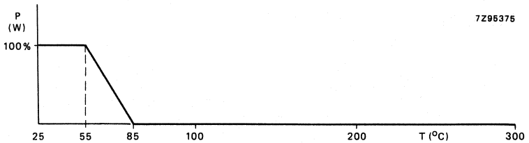
Fig. 2 Derating curve.
