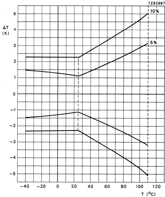
Fig. 4 Temperature deviation (in K) over the range from -40 °C to 110 °C for both 5% and 10% thermistors.
