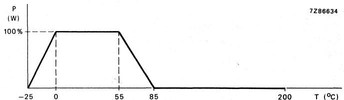
Fig. 2 Derating curve.
