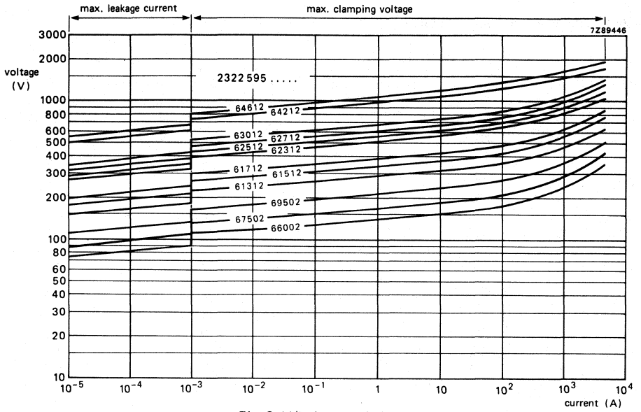
Fig. 2 V/I characteristics.
