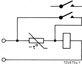
Fig. 18 Delaying action of relays. Due to the thermal inertia of the NTC, it takes some time before the relay is activated. If necessary the NTC can be short-circuited after the relay is activated thus leaving the NTC time for cooling.
