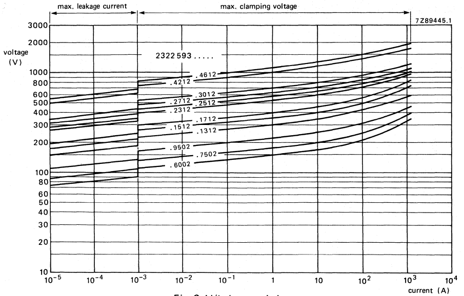
Fig. 2 V/I characteristics.
