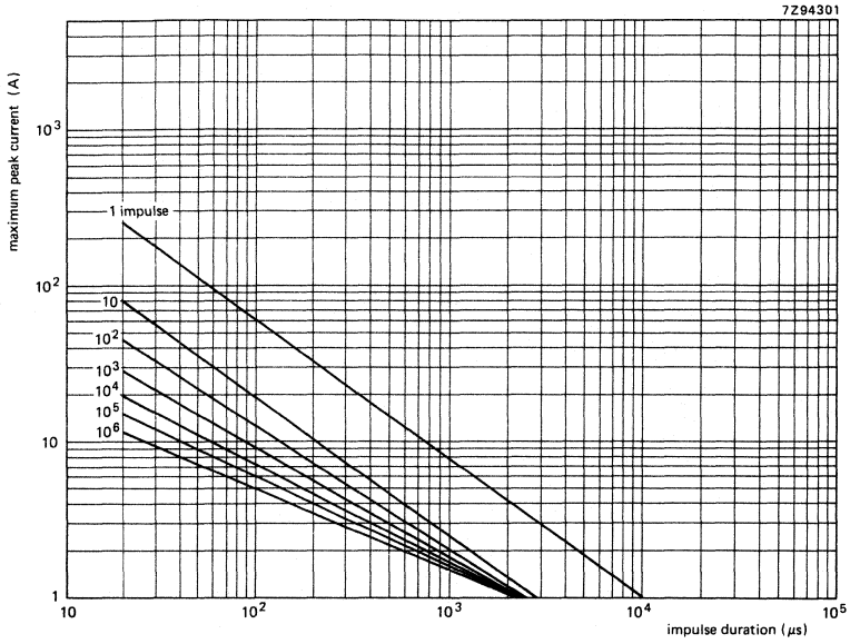
Fig. 15 Max. applicable transient current as a function of impulse duration, 30/40 V, 593 series.
