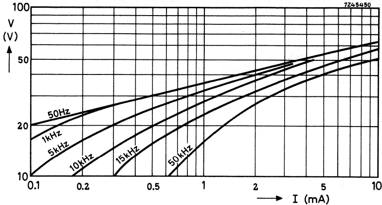
Fig. 8 Voltage/current relation for different frequencies.
