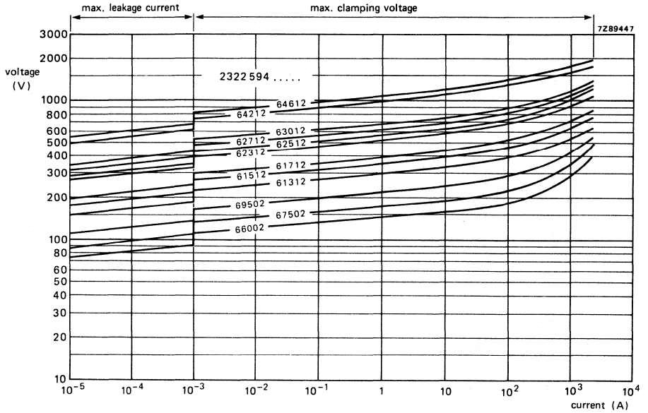
Fig. 2 V/I characteristics.
