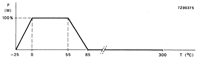
Fig. 2 Derating curve.
