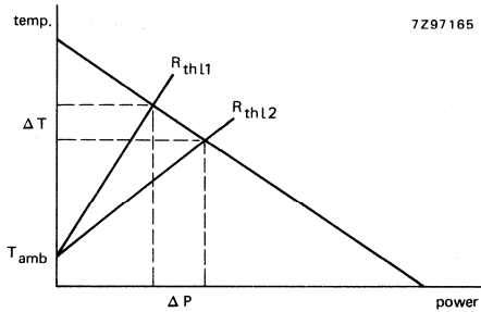
Fig. 5 Influence of load variation.
