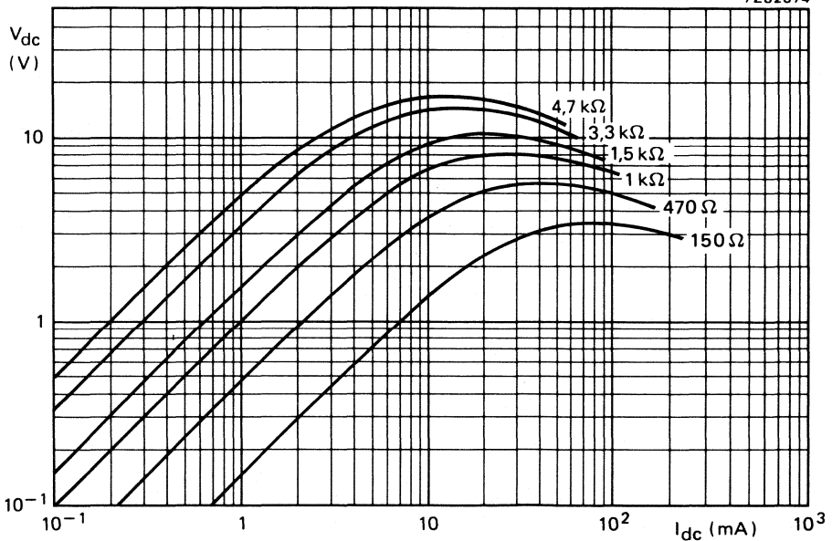
Fig. 6 Typical voltage/current characteristic, T_{amb} = +25\text{ }^{\circ}\text{C} , still air.
