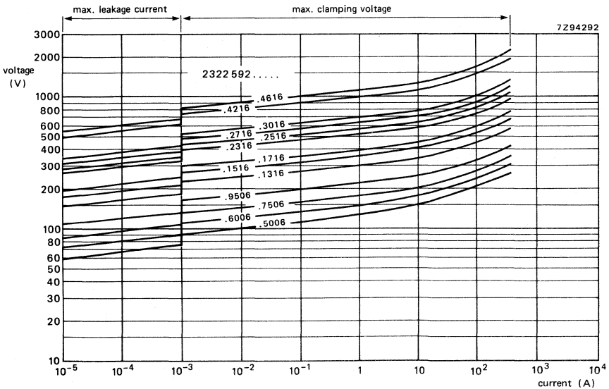
Fig. 6 V/I characteristics, 50/460 V, 592 series.
