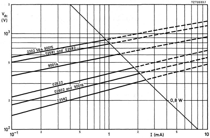
Fig. 2 Voltage/current characteristics.
