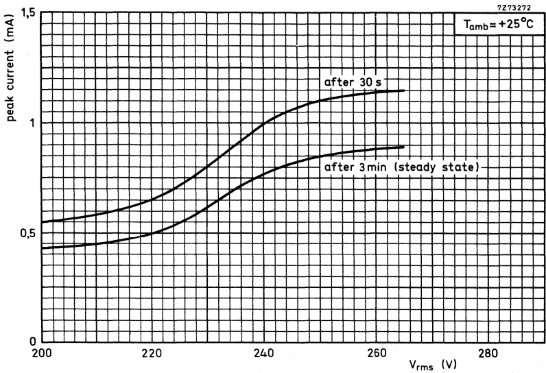
Fig. 8 Typical peak current versus voltage characteristics.
