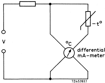
Fig. 13 Temperature measurement in cars. Cooling water measurements with bimetal or differential millimeters.
